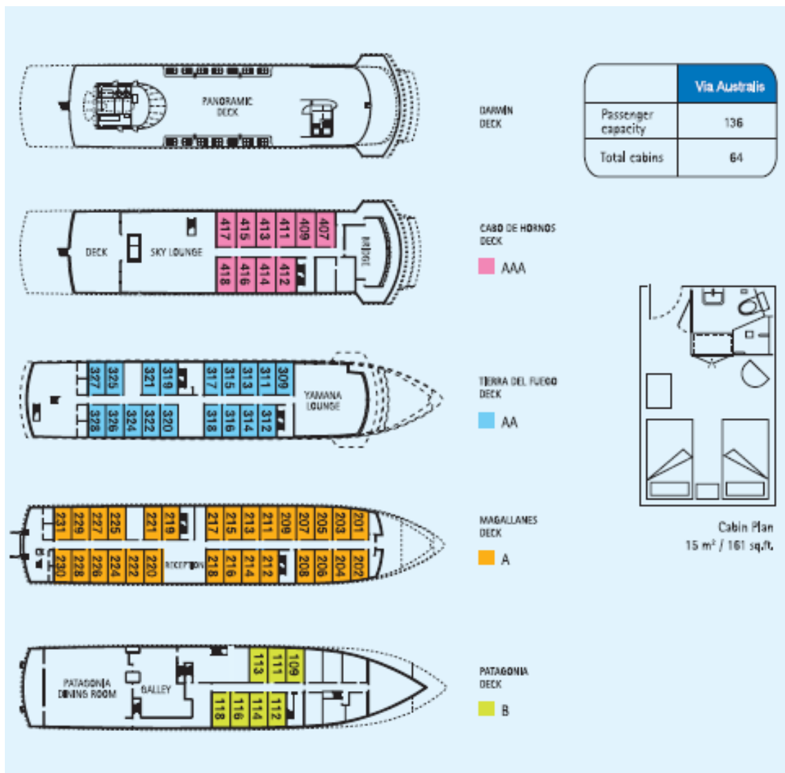
Deck Plan Via Australis
