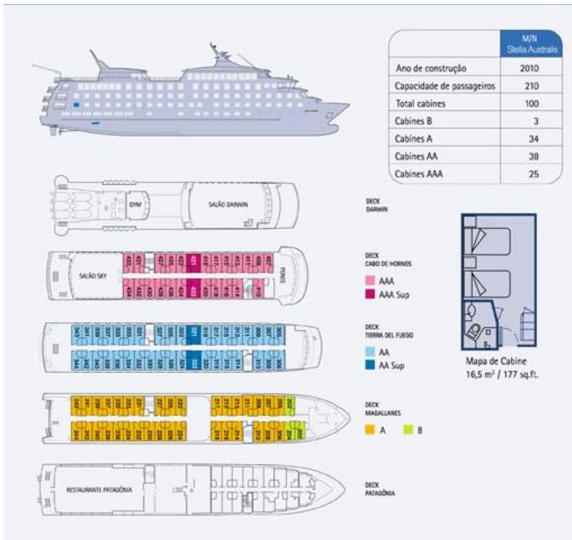
Deck Plan Stella Australis
